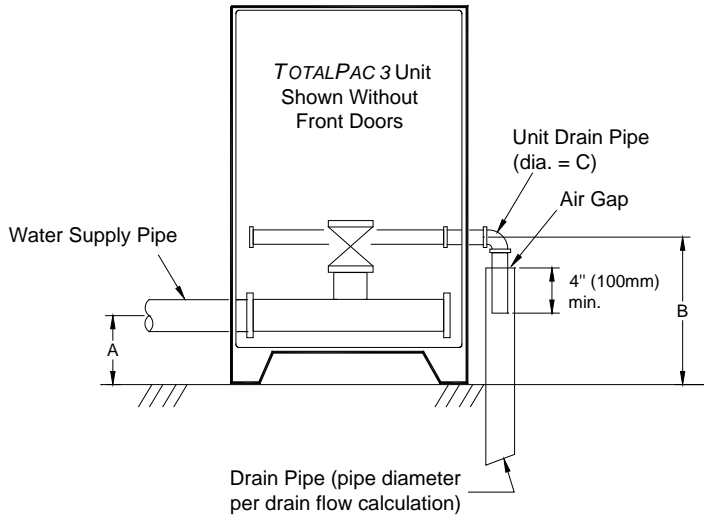
Figure 5 - Open drain details for single unit
