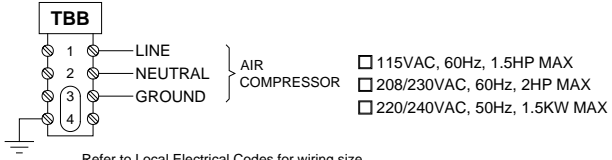
WIRING OF AIR COMPRESSOR POWER SOURCE (WITH AIR OPTION "C" ONLY)
