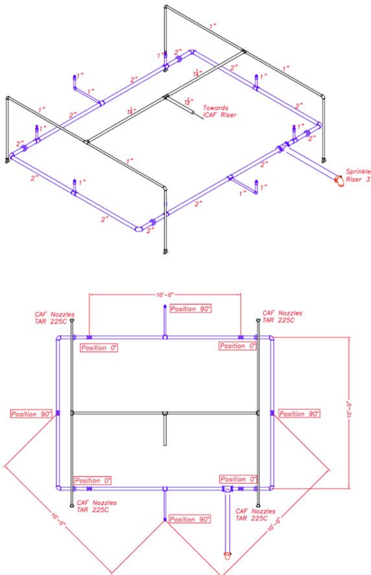
Figure 1. CAF and Sprinkler Piping Layout and CAF Generator
