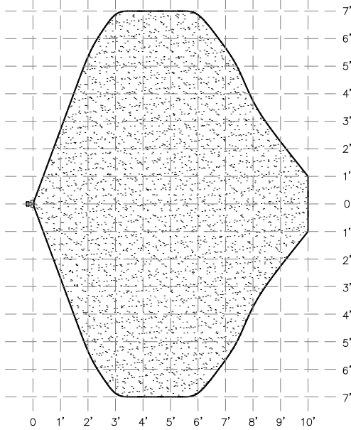
HORIZONTAL DISCHARGE
